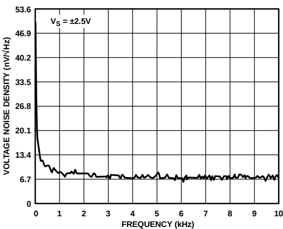
Figure 29. Voltage Noise Density vs. Frequency
