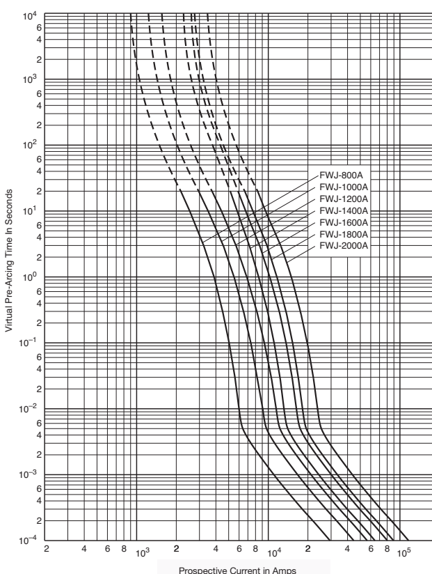
Time-Current Curve
