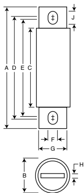
Fig. 1: 5-800A
