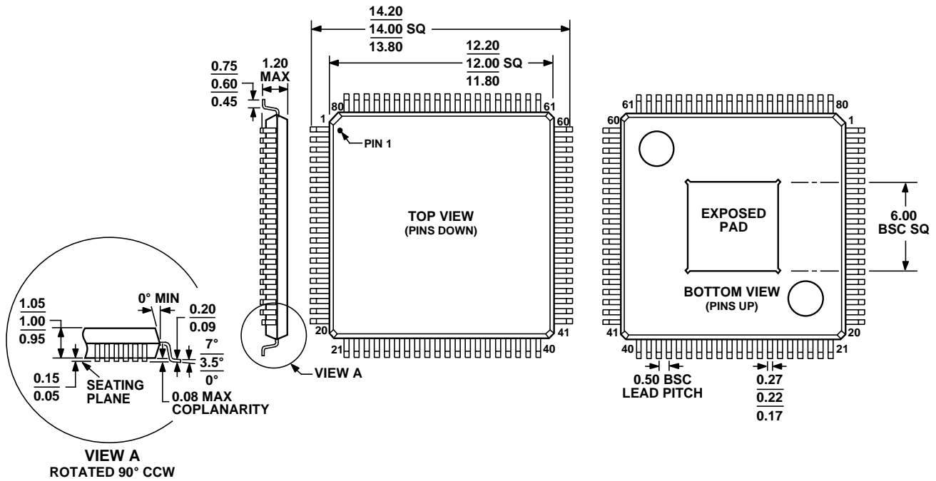
COMPLIANT TO JEDEC STANDARDS MS-026-ADD-HD Figure 21. 80-Lead Thin Quad Flat Package, Exposed Pad [TQFP_EP] (SV-80-1) Dimensions shown in millimeters
