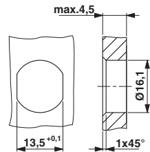
Mounting cutout with polarization for M16 thread
