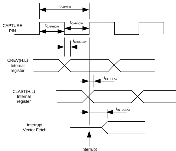
Figure 10 CAPTURE timing
