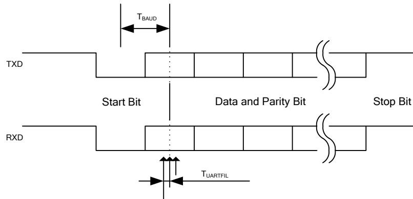
Figure 9 UART timing
