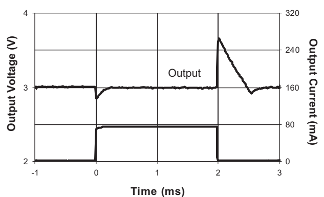
Load Transient - 1mA / 80mA
