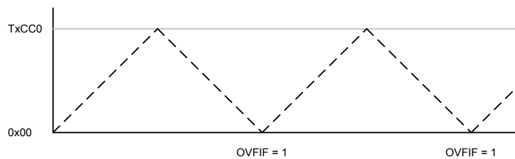
Figure 38: Up/Down Mode
