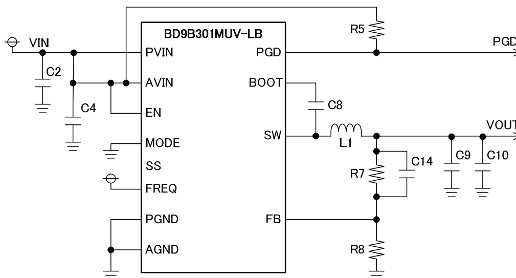
Figure 48. Application Circuit
