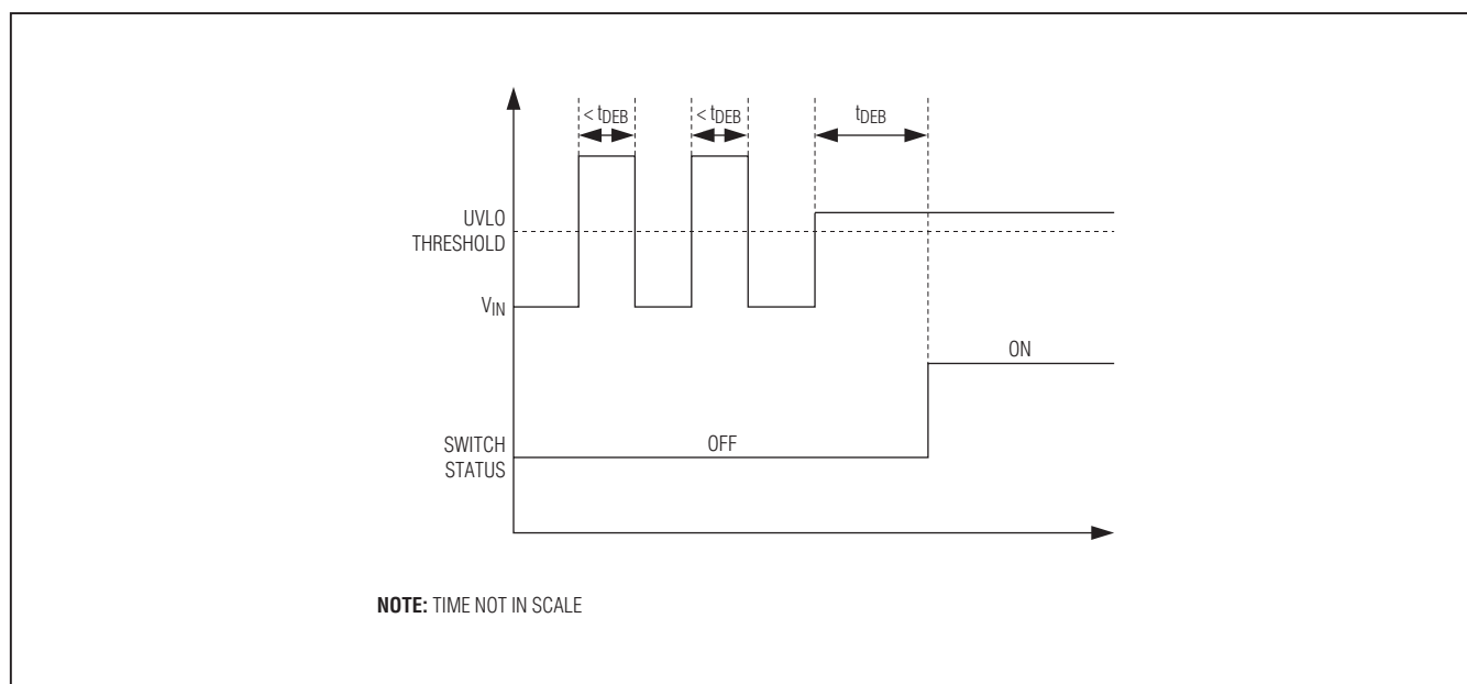
Figure 4. Debounce Timing
