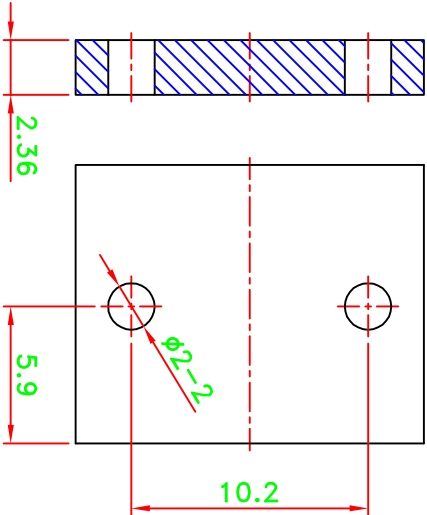
PCB MOUNTING HOLE
