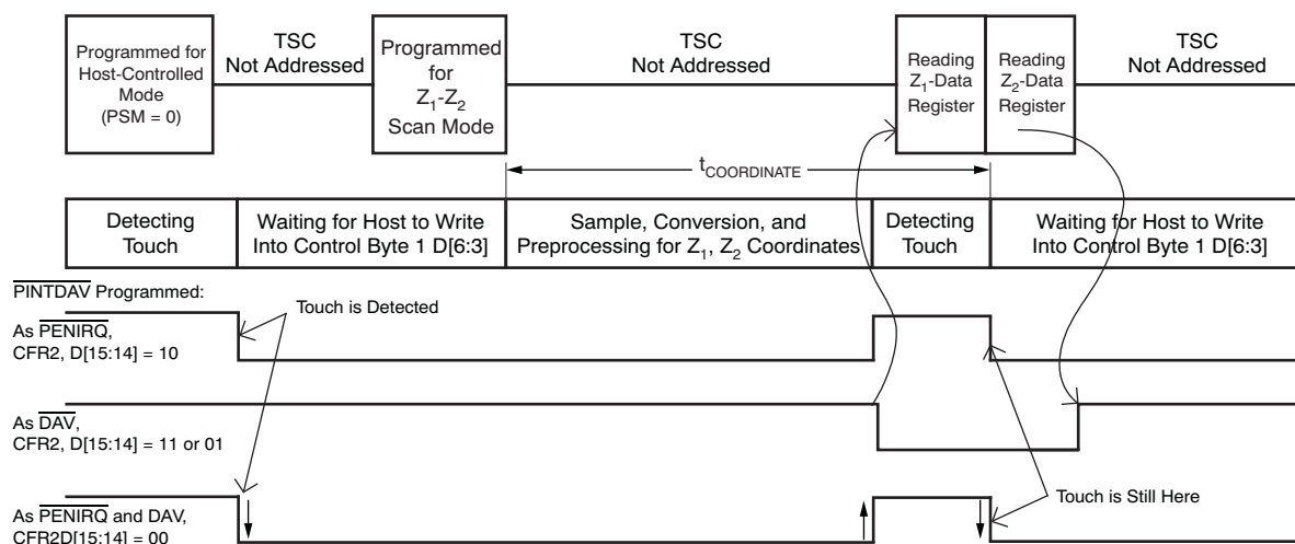
Figure 44. Example of a Z_1 and Z_2 Coordinate Touch Screen Scan (with Panel Stabilization Time) using TSMODE 3
