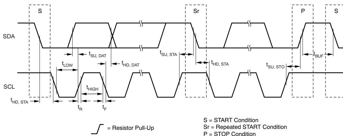
Figure 1. Detailed I/O Timing for Standard and Fast Modes
