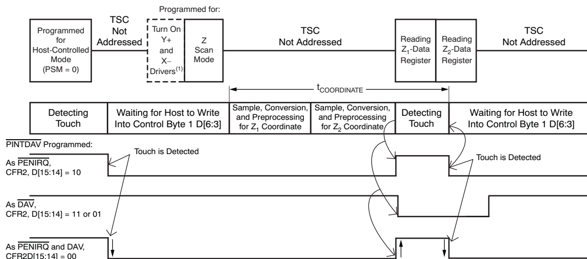
Figure 43. Example of Z_1 and Z_2 Coordinate Touch Screen Scan (without Panel Stabilization Time) using TSMODE 3
