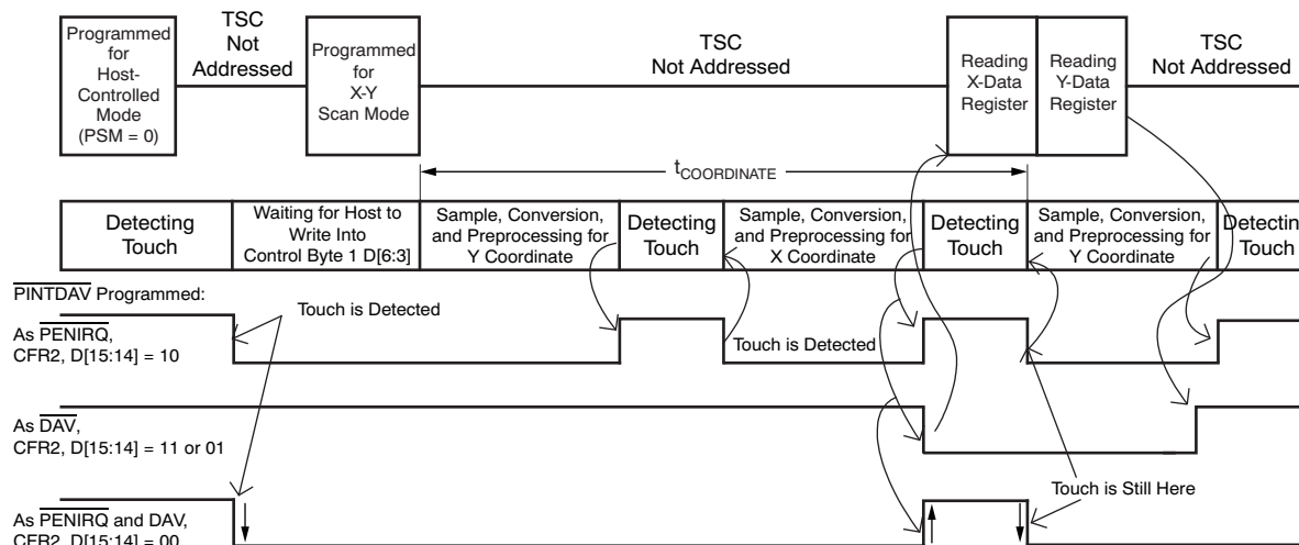
Figure 41. Example of an X and Y Coordinate Touch Screen Scan using TSMODE 2
