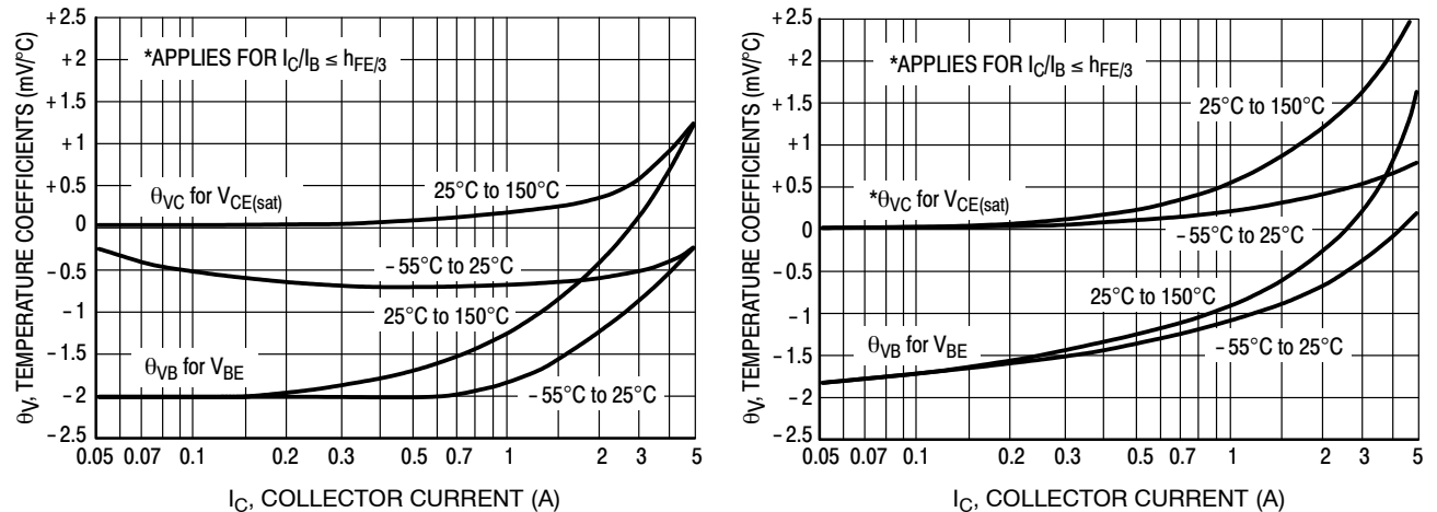
Figure 7. Temperature Coefficients
