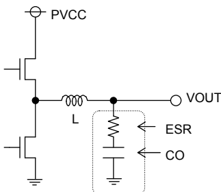
Figure 41. Output capacitor
