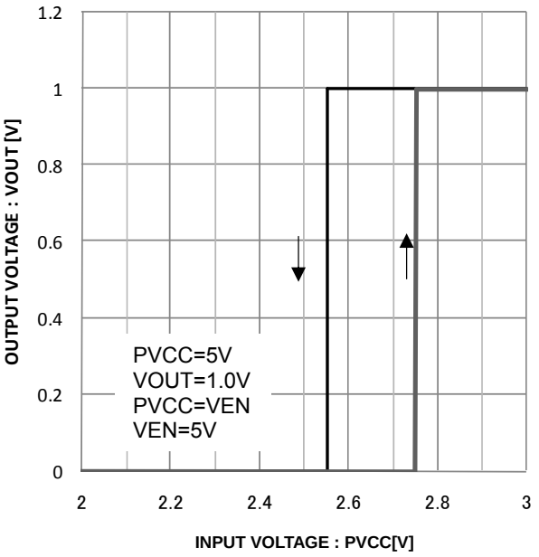
Figure 22. PVCC start-up
