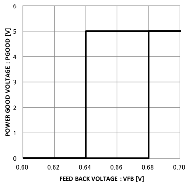
Figure 26. PowerGood voltage/hysteresis
