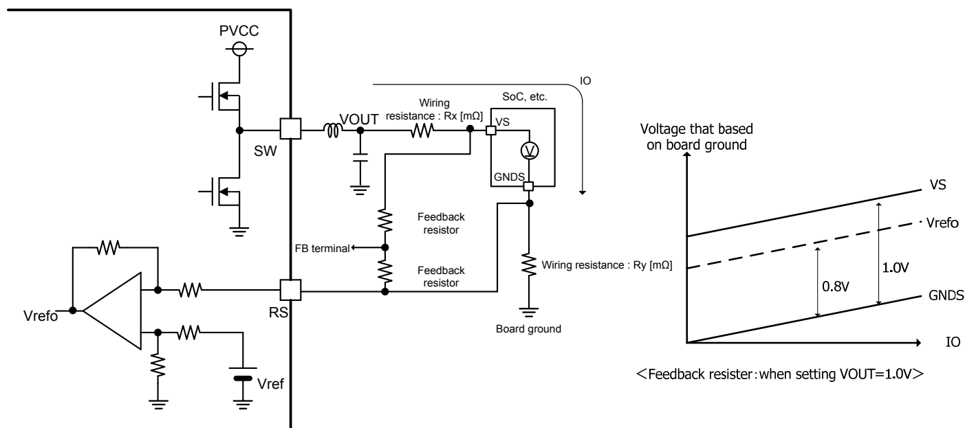
Figure 38. Remote sense
