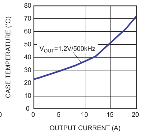
Thermal Results
