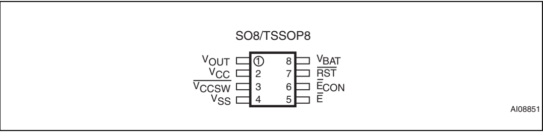
Figure 6. STM795 connections
