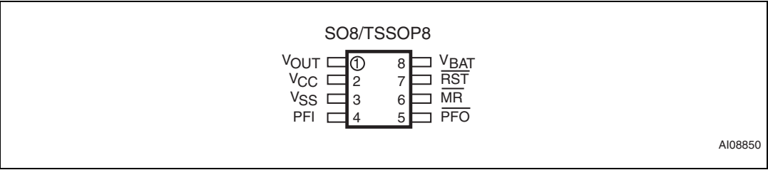
Figure 5. STM704/806 connections
