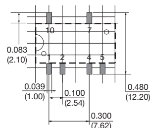
Recommended Footprint Top View grid: 0.1 x 0.1 in (2.54 x 2.54 mm)
