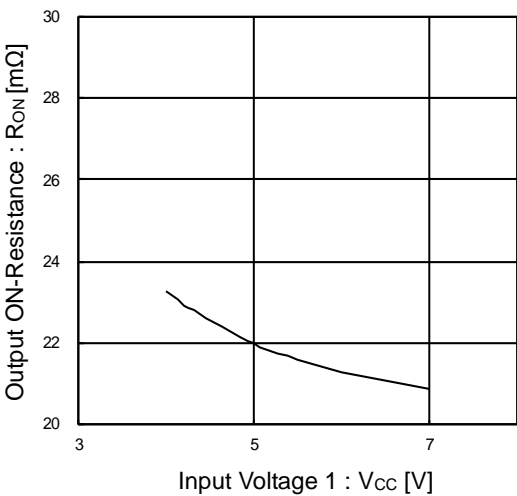
Figure 22. Output ON-Resistance vs Input Voltage 1 (VOUT=1.5V)
