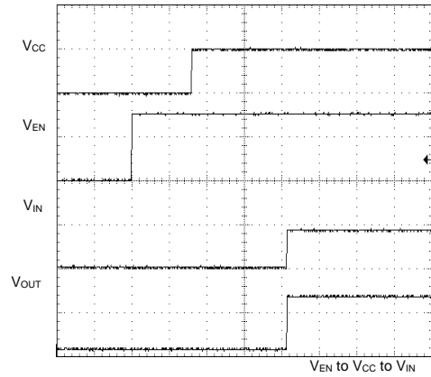
Figure 11. Input Sequence
