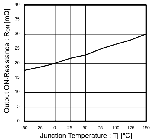
Figure 21. Output ON-Resistance vs Junction Temperature (VCC=5V/VOUT=1.5V)
