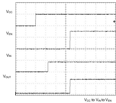
Figure 9. Input Sequence
