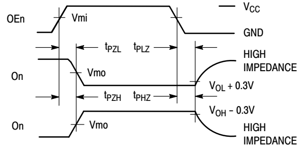
WAVEFORM 2 – OUTPUT ENABLE AND DISABLE TIMES
