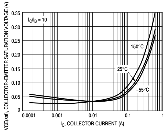
Figure 3. Collector-Emmitter Saturation Voltage vs. Collector Current
