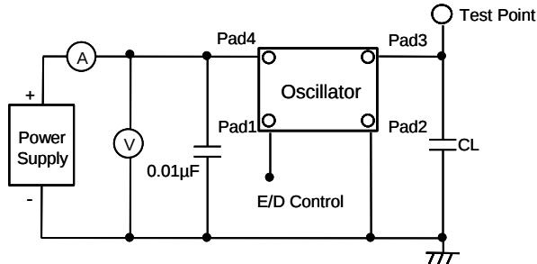
Fig.1 Test Circuits
