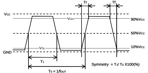
Fig.2 Clock Timing Chart (C-MOS Output)
