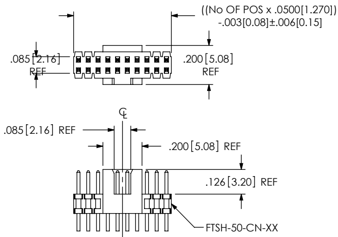
FIG 7 -K OPTION (LEAD STYLE -01) (DIFFERENT AS SHOWN, OTHERWISE SAME AS FIG 1) (POSITION 13, 17, 20 & 25 AVAILABLE WITH -K & -EJ OPTION)
