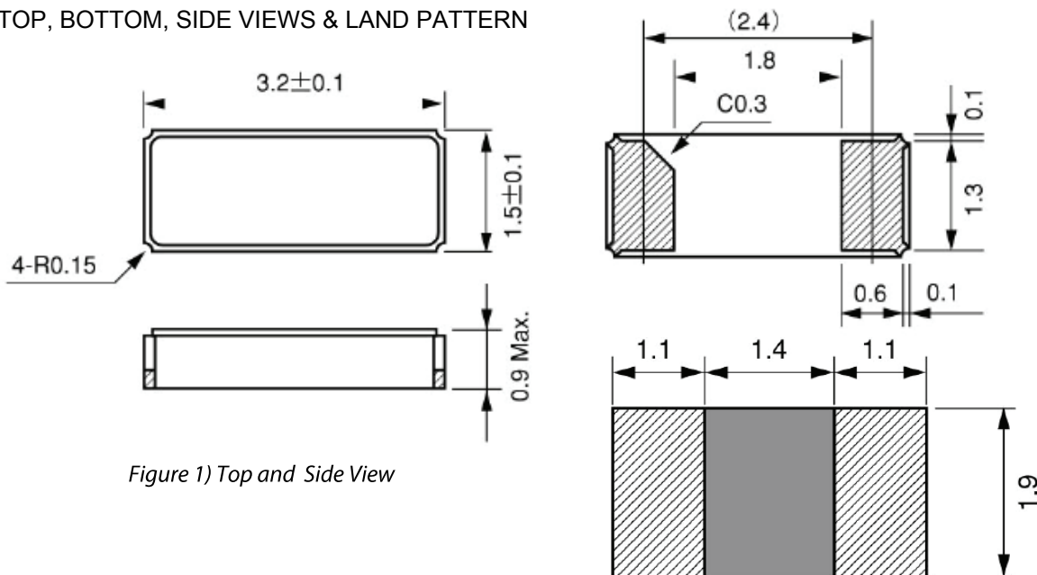
Figure 2) Bottom View and Suggested Land
