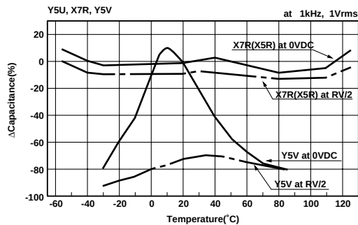
Capacitance-Temperature (high dielectric constant)
