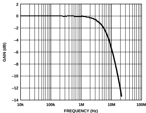
Figure 3. Reference Multiplying Bandwidth
