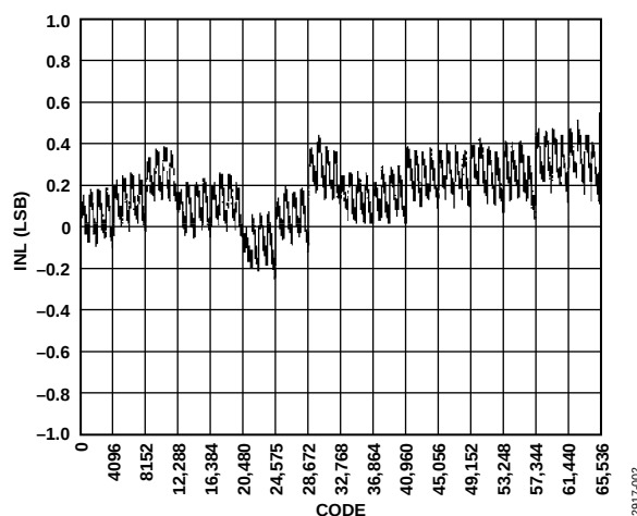
Figure 2. Integral Nonlinearity
