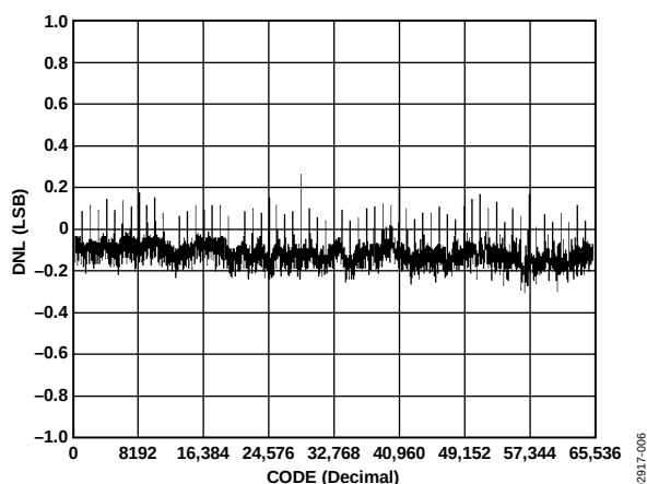
Figure 8. AD5543 Differential Nonlinearity Error
