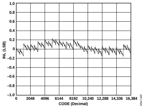
Figure 9. AD5553 Integral Nonlinearity Error
