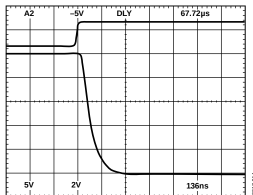
Figure 16. Settling Time
