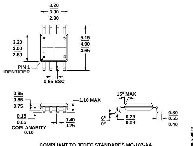
Figure 32. 8-Lead Mini Small Outline Package [MSOP] (RM-8)
