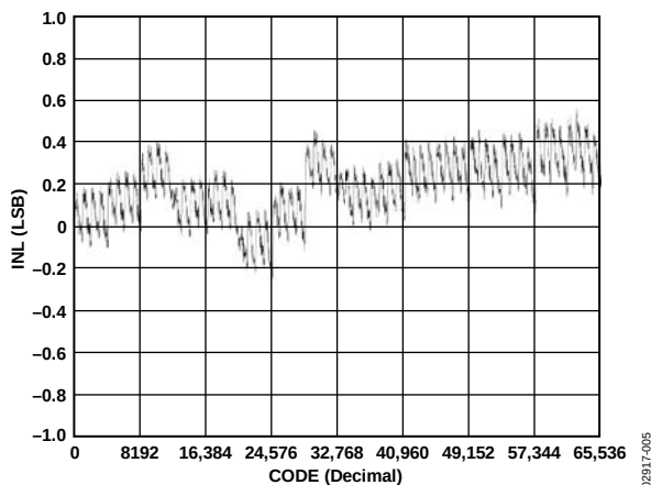
Figure 7. AD5543 Integral Nonlinearity Error
