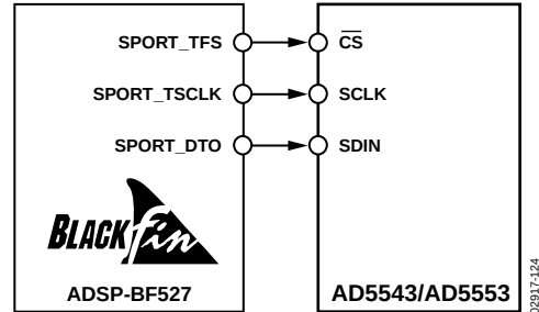
Figure 25. AD5543/AD5553 to SPORT Interface
