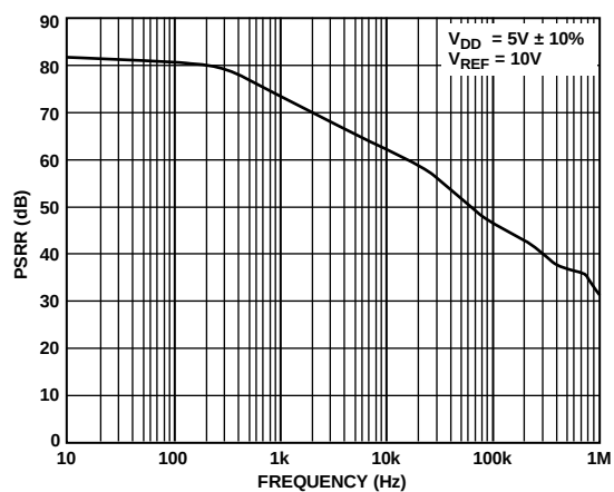
Figure 14. Power Supply Rejection Ratio (PSRR) vs. Frequency
