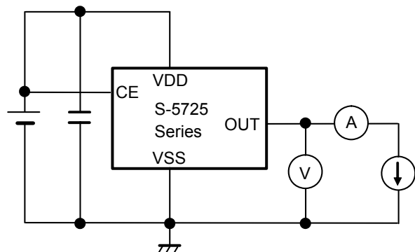
Figure 15 Test Circuit 3
