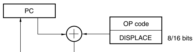
Figure 3-28. Outline of Relative Addressing
