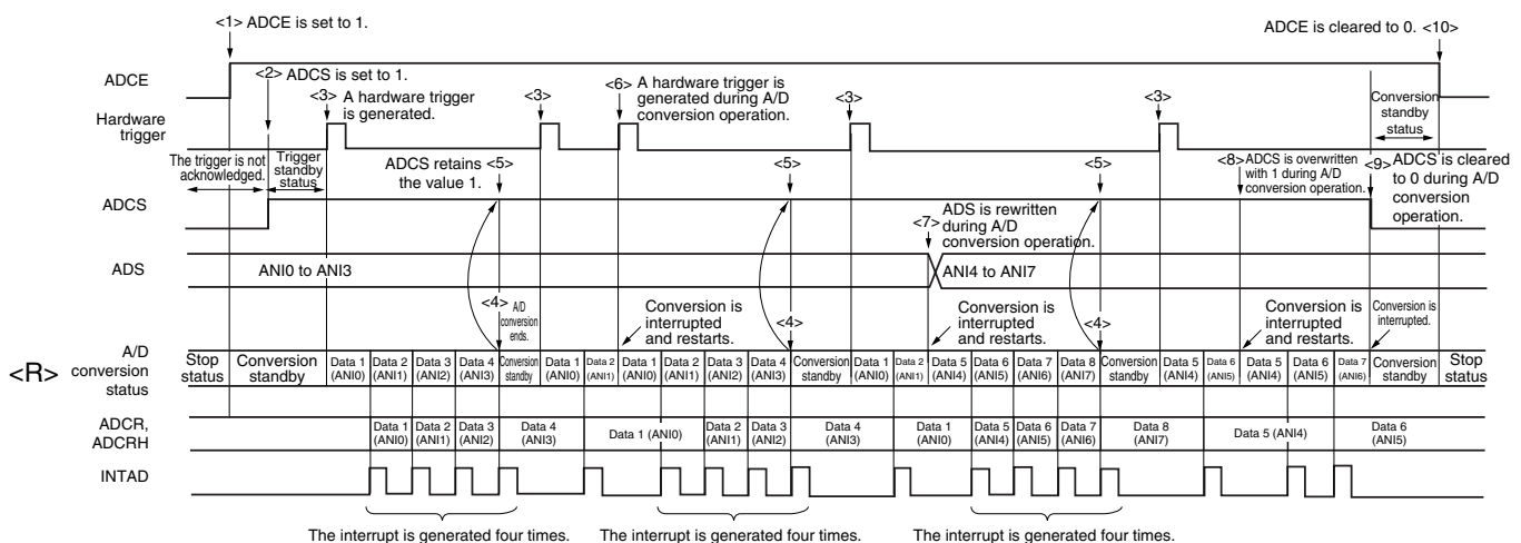
Figure 11-27. Example of Hardware Trigger No-Wait Mode (Scan Mode, One-Shot Conversion Mode) Operation Timing
