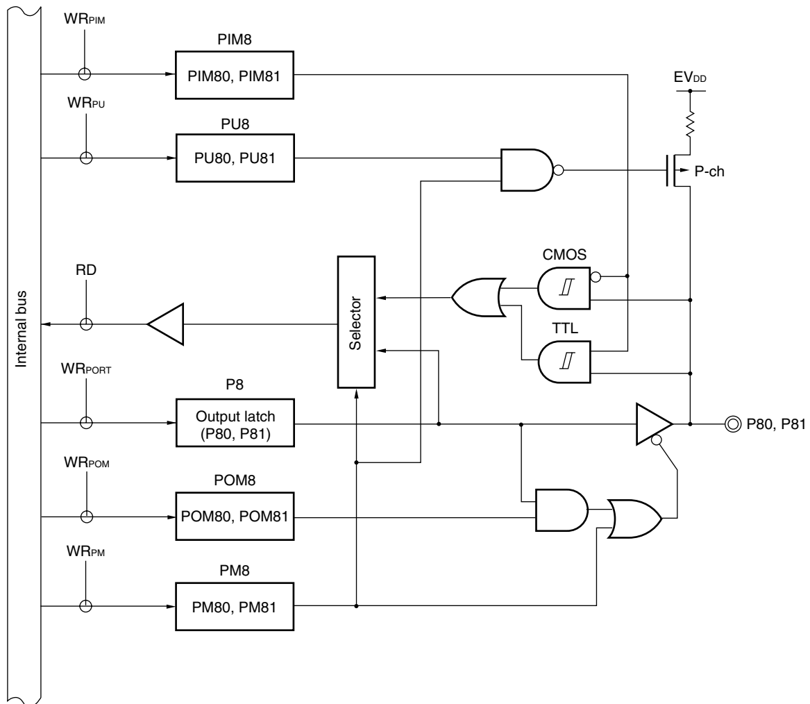
Figure 4-39. Block Diagram of P80, P81
