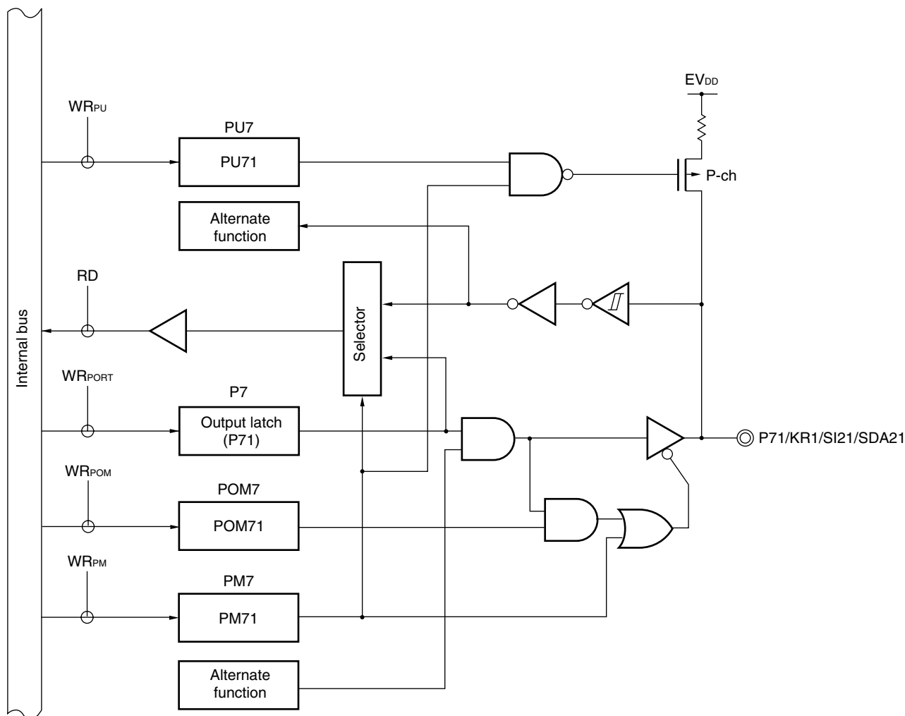
Figure 4-35. Block Diagram of P71
