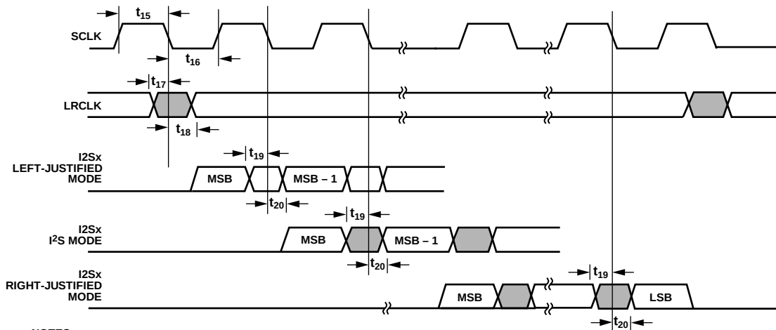
Figure 6. I²S Timing
