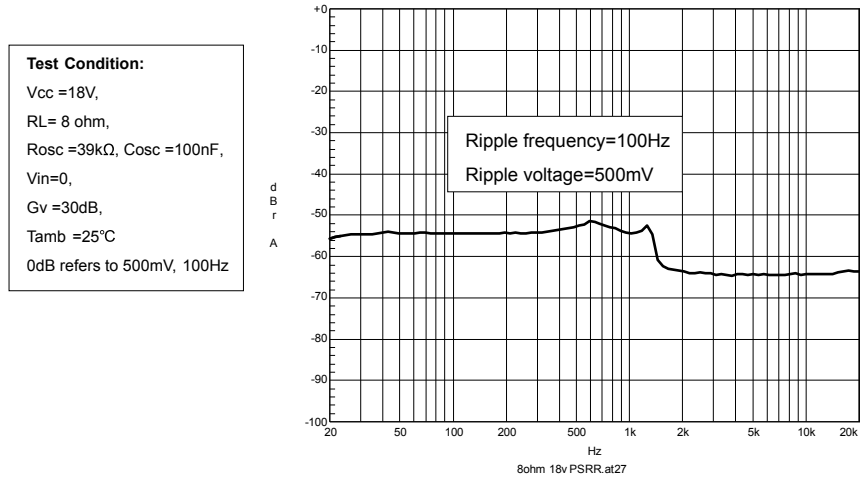
Figure 42. Power supply rejection ratio vs. frequency
