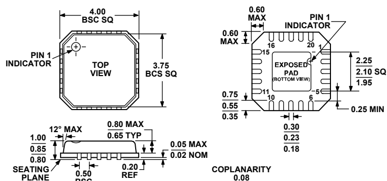
Figure 24. 20-Lead Lead Frame Chip Scale Package [LFCSP_VQ] 4 mm × 4 mm Body, Very Thin Quad (CP-20-1)
