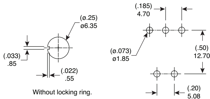
Panel Mounting
