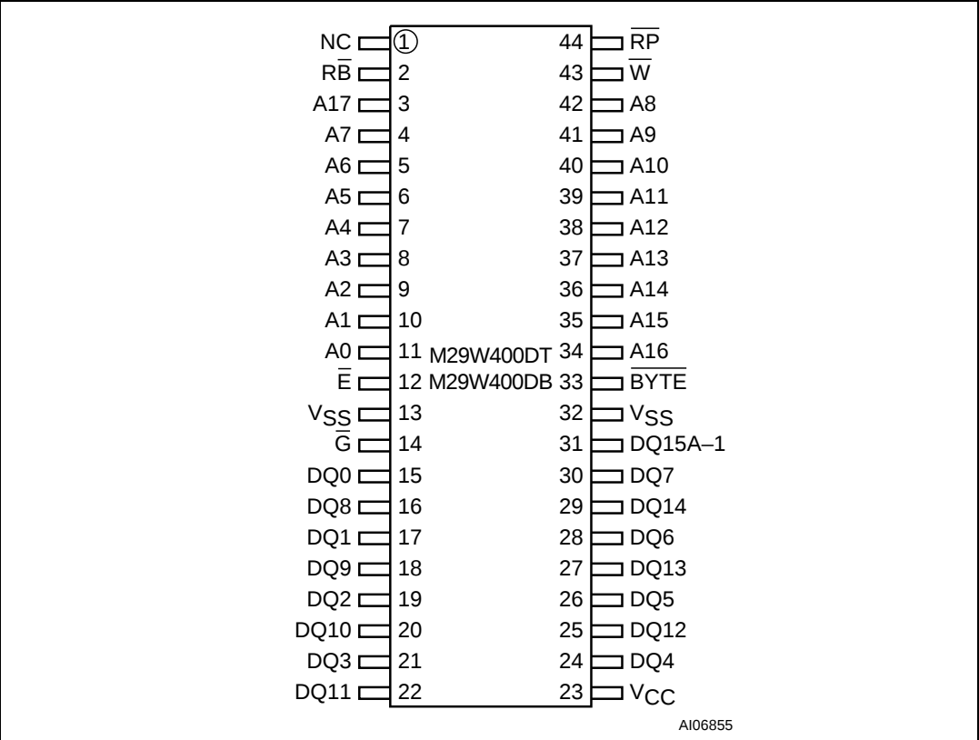
Figure 2. SO connections
