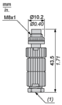
(1) Cable gland : M9.5 x 1
