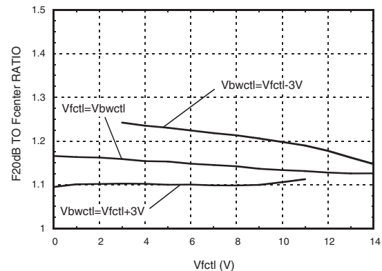
High Side Rejection Ratio vs. Bandwidth Control [1]
