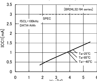
Fig.13 Current consumption at WRITE action ICC1 ( f_{SCL}=100\text{kHz} )
