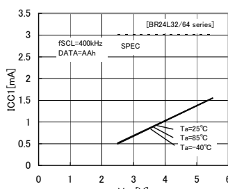
Fig.10 Current consumption at WRITE action ICC1 ( f_{SCL}=400\text{kHz} )
