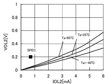
Fig.6 L output voltage V_{OL,2} - I_{OL,2} ( V_{CC}=1.8\text{V} )
