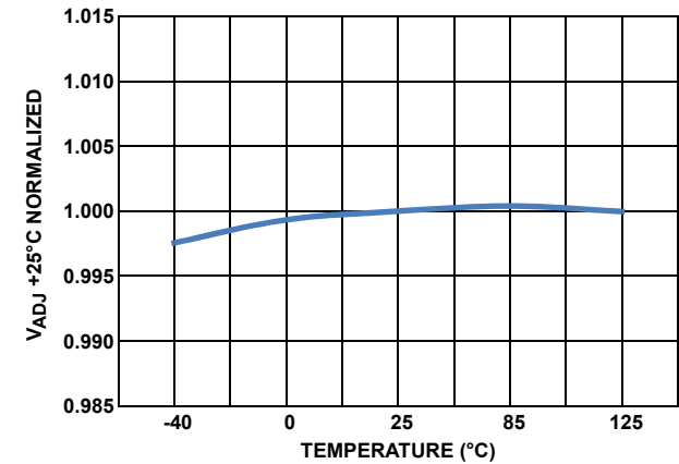
FIGURE 8. V_{ADJ} vs TEMPERATURE
