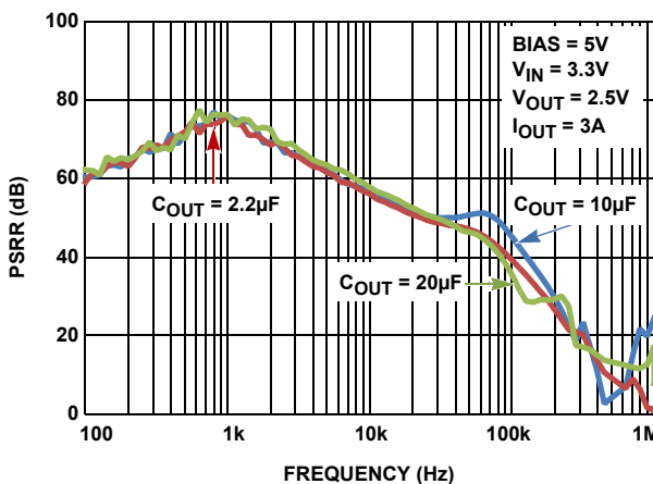
FIGURE 32. V_{\text{IN}} PSRR vs FREQUENCY FOR VARIOUS C_{\text{OUT}}
