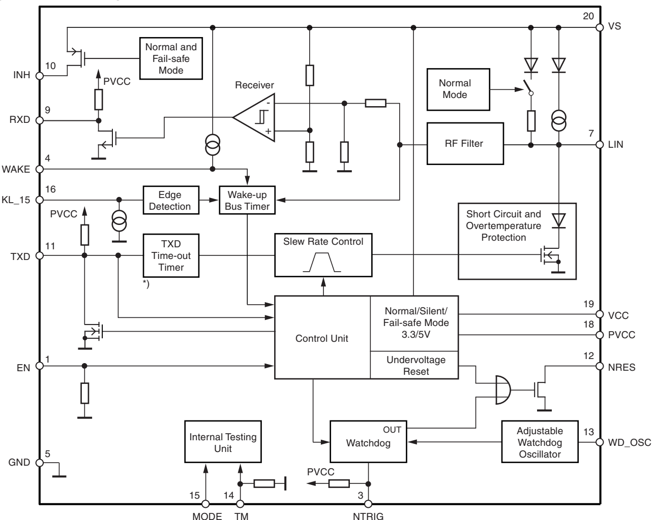
Figure 1-1. Block Diagram
