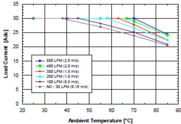
Fig. 2.5V.1: Available load current vs. ambient air temperature and airflow rates for SQE48T30025 converter mounted vertically with air flowing from pin 3 to pin 1, MOSFET temperature ≤ 120 °C, Vin = 48 V.
