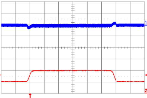
Fig. 1.2V.9: Output voltage response to load current step-change (10 A – 20 A – 10 A) at V_{in} = 48\text{ V} . Top trace: output voltage (100 mV/div.). Bottom trace: load current (10 A/div.). Current slew rate: 0.1 A/ \mu\text{s} . C_o = 1\text{ }\mu\text{F} ceramic. Time scale: 0.2 ms/div.
