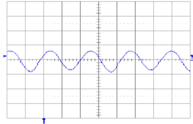
Fig. 2.5V.13: Input reflected-ripple current, c (100 mA/div.), measured at input terminals at full rated load current and V_{in} = 48 \text{ V} . Refer to Fig. 2.5V.12 for test setup. Time scale: 1 \mu\text{s}/\text{div} .
