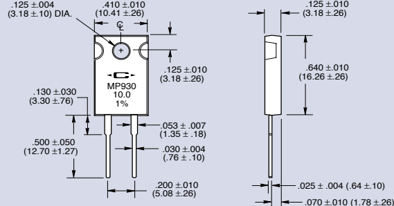
Figure 2 TO-220 Style MP916, MP925 and MP930
