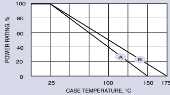
Derating Curve
