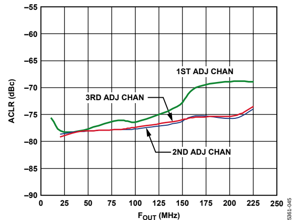
Figure 48. AD9776 ACLR, f_{\text{DATA}} = 122.88\text{ MSPS} , 4 \times Interpolation, f_{\text{DAC}}/4 Modulation
