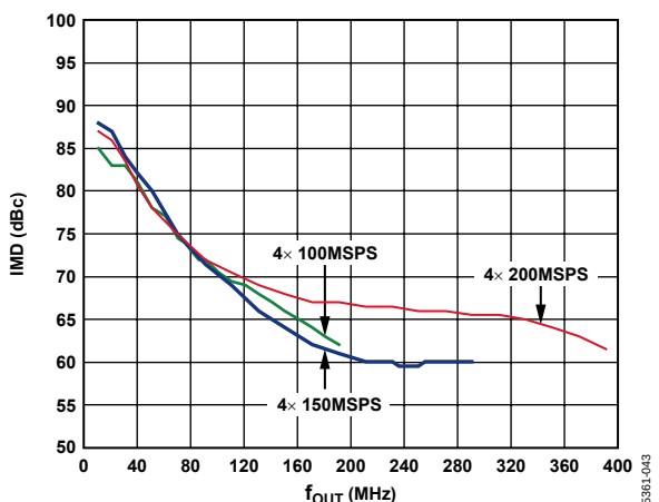
Figure 46. AD9776 IMD, 4 \times Interpolation
