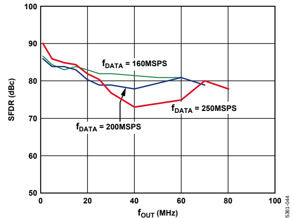
Figure 47. AD9776 In-Band SFDR, 2 \times Interpolation
