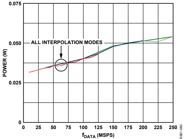
Figure 84. Digital 3.3 V Supply, I Data Only, Real Mode, Includes Modulation Modes and Zero Stuffing
