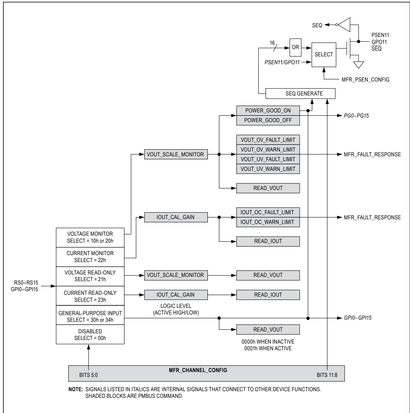
Figure 12. MFR_CHANNEL_CONFIG Command
