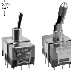
Straight PC • Bracket Four Pole
