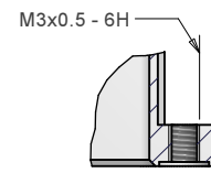
HARDWARE OPTION M3-0 (THREADED HOLES M3)
