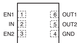
TLV710 TLV711 1.5mm × 1.5mm SON-6 (TOP VIEW)
