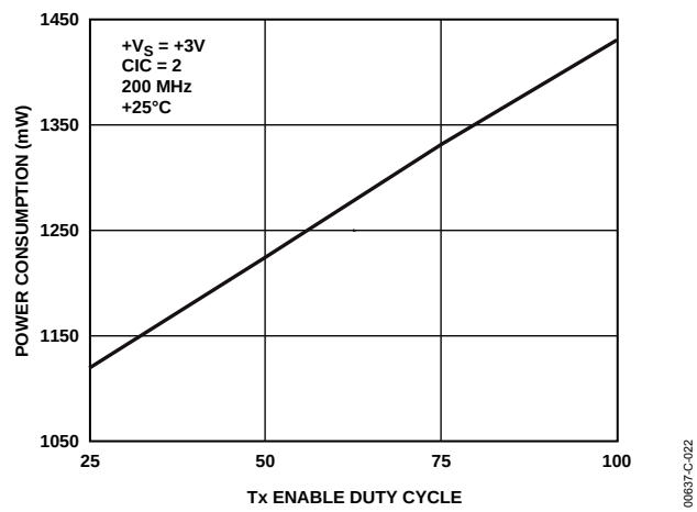
Figure 22. Power Consumption vs. Burst Duty Cycle; V_S = 3\text{ V} , CIC = 2 , 200\text{ MHz} , 25^\circ C
