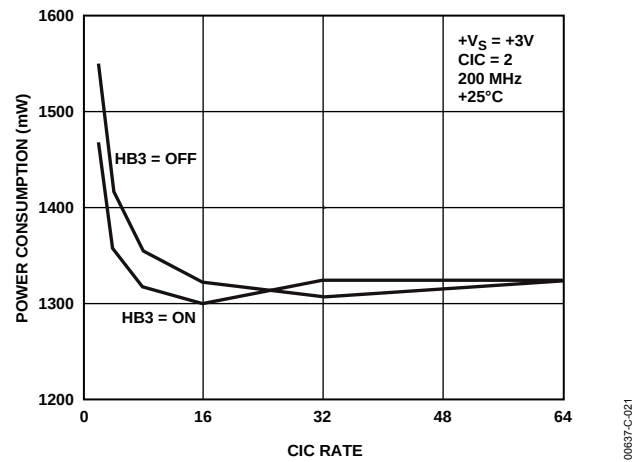
Figure 21. Power Consumption vs. CIC Rate; V_S = 3\text{ V} , 200\text{ MHz} , 2^\circ C
