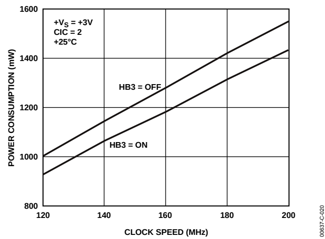
Figure 20. Power Consumption vs. Clock Speed; V_S = 3\text{ V} , CIC = 2 , 25^\circ C
